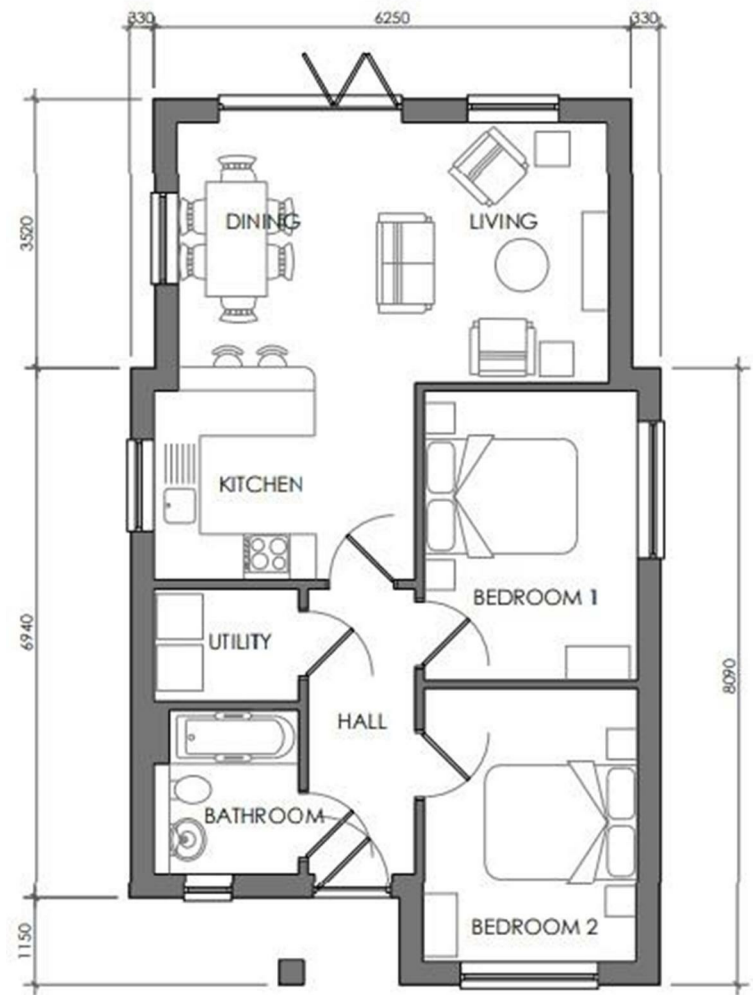
FLOOR PLAN GROSS INTERNAL FLOOR AREA = 63.23m.sq. (681sq.ft.)
